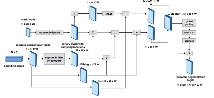
Fig. 4: Panoptic head. Panoptic masks logits are constructed by adding the instance masks logits with the semantic logits. Sampling locations in the object bounding box are determined by prominent features from the semantic logits at category level.
