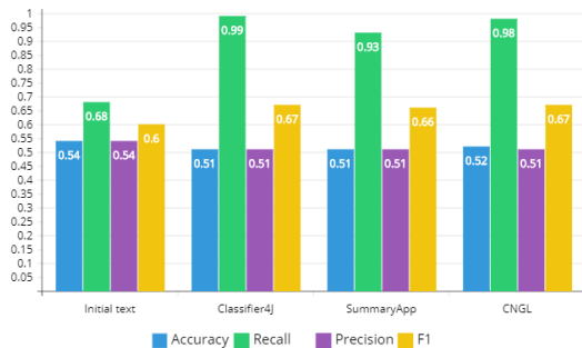
Fig. 3: Results on the training corpus <T, T_{summarize}> .
