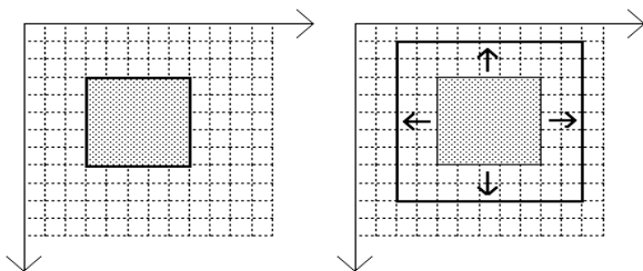
Figure 2. Inter-correlation principle
