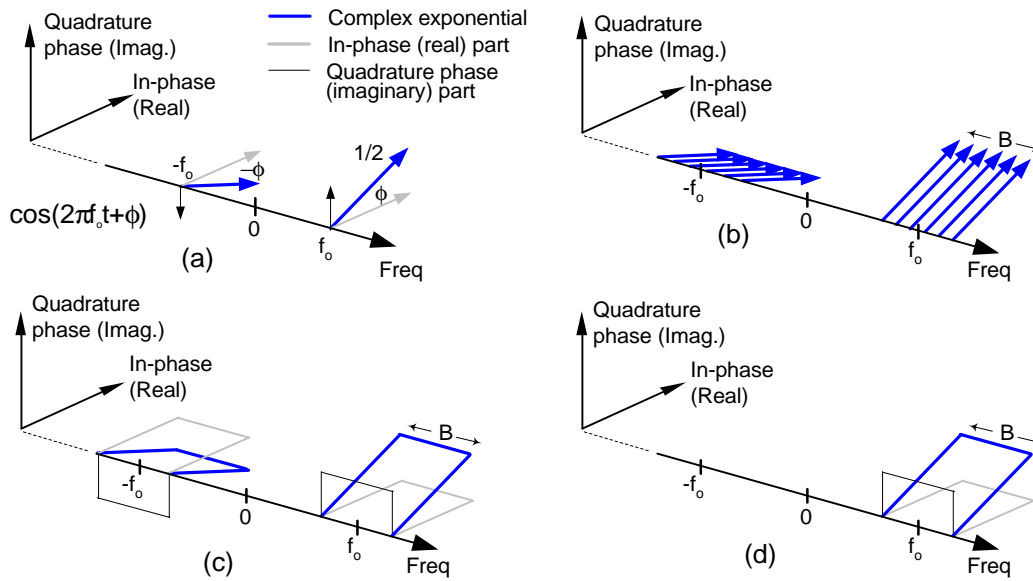
Figure 11. Quadrature representation of signals: (a) Real sinusoid \cos(2\pi f_0 t + \phi) , (b) Real bandpass signal containing seven sinusoids over bandwidth B ; (c) Real bandpass signal containing an infinite number of sinusoids over bandwidth B Hz; (d) Complex bandpass signal of bandwidth B Hz.
