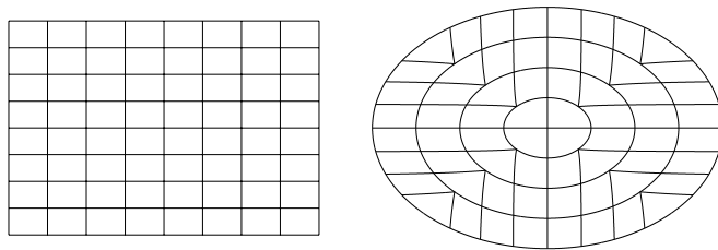
FIGURE 2. A uniform grid on a rectangle and its image - a uniform grid on the elliptic domain.
