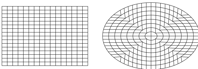
FIGURE 3. A refinement of the grid in Figure 2 and its image - a refinement of the elliptic grid in Figure 2.
