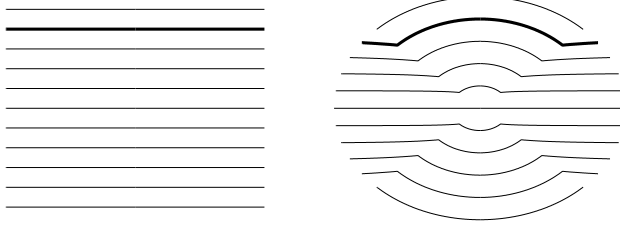
FIGURE 1. A horizontal grid and its image grid on the elliptic domain. The image of the bold line on the left is the bold curve on the right.
