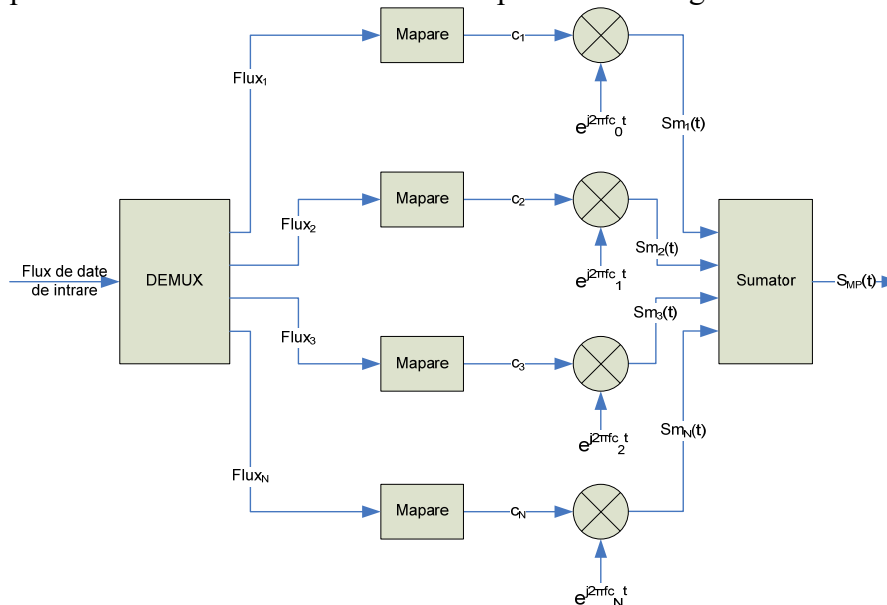
Figura 2 Modulator OFDM-BB
