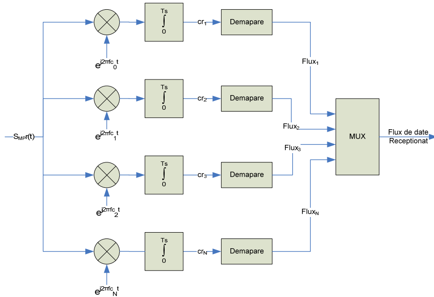
Figura 3. Demodulator OFDM-BB
