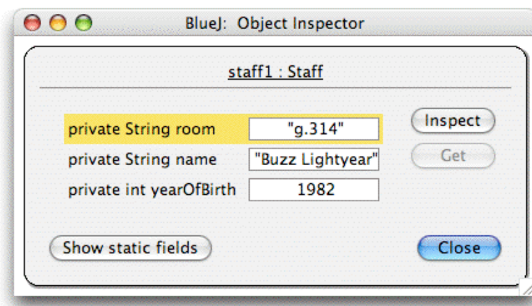
Figure 9: Inspection dialogue
