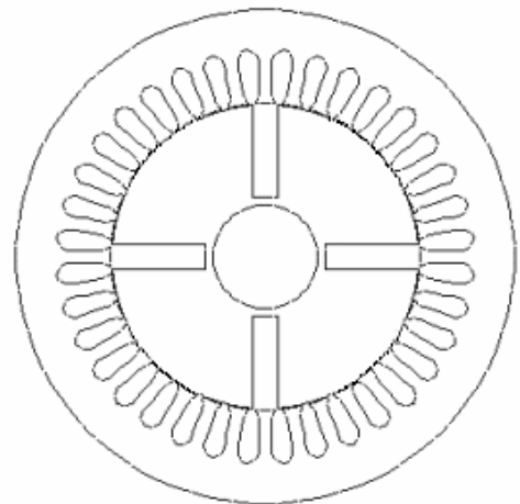
Fig. 1. The motor's structure
