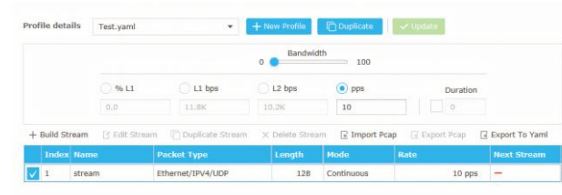
Figure 9. Traffic profile of the TRex
