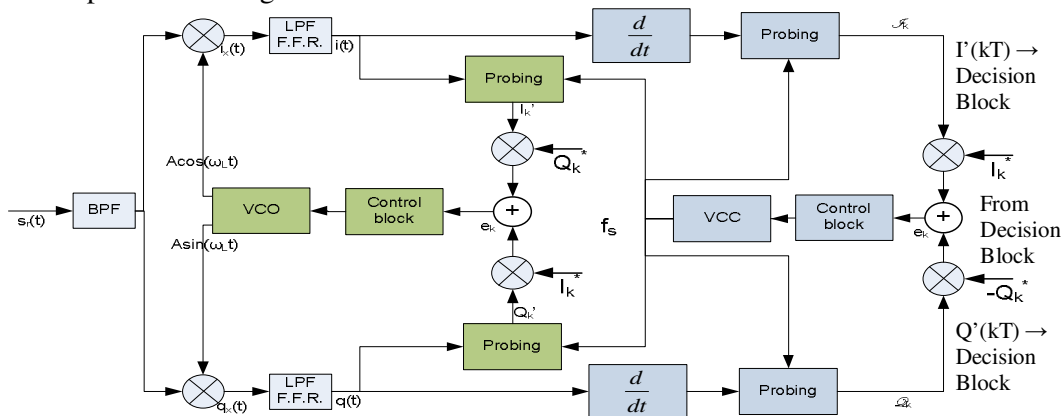
Figure 9. DD-based recovery and synchronization of the local carrier and symbol clock
