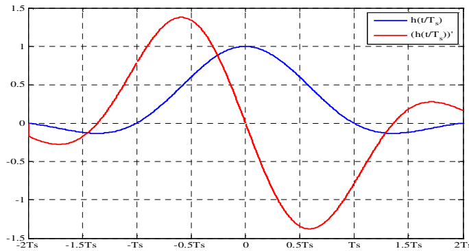
Fig.8 Impulse response of the RC filter (blue) and its first order derivative (red)
