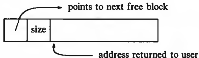
A block returned by malloc
