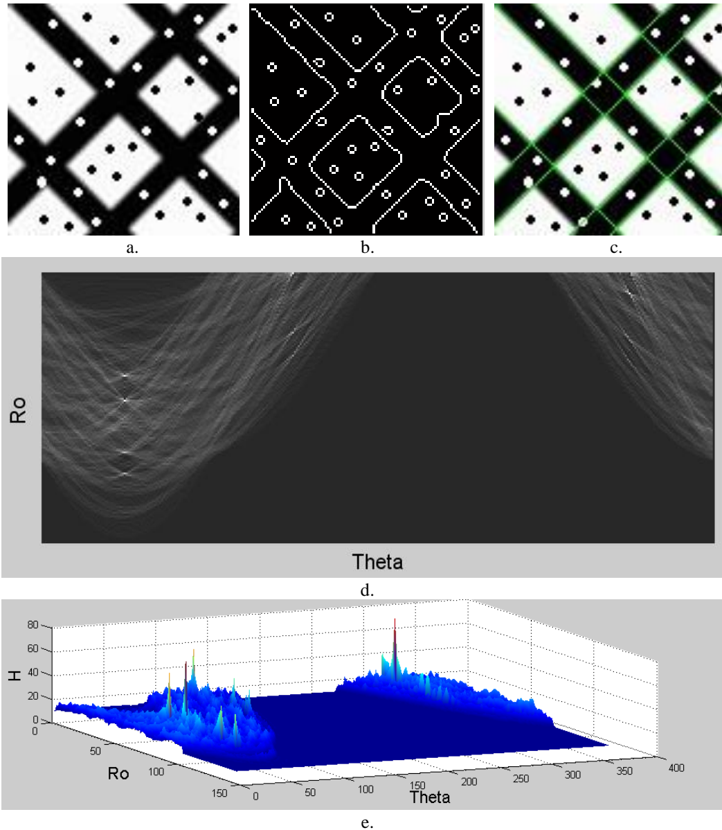
Fig. 2. a. An image containing a pattern with straight borders corrupted by salt-and-pepper like noise, b. The edges detected with the Canny edge detector, c. The most relevant image lines are displayed with green, associated to the most relevant 8 peaks from the Hough accumulator, d. The Hough accumulator displayed using an intensity encoding, e. The Hough accumulator displayed in 3D, using color encoding.
