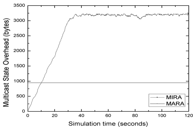
Fig. 6. Multicast state behaviour
