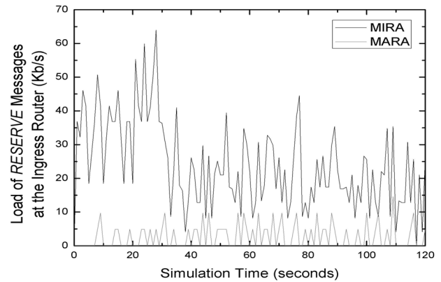
Fig. 5. Load of RESERVE messages
