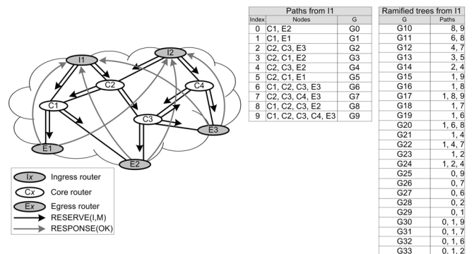
Fig. 3. List of all multicast aggregation trees created by MARA
