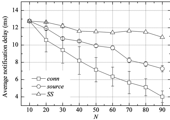
Fig. 13. Notification delay versus offered load.
