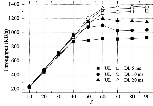
Fig. 2. Throughput versus number of SSs.
