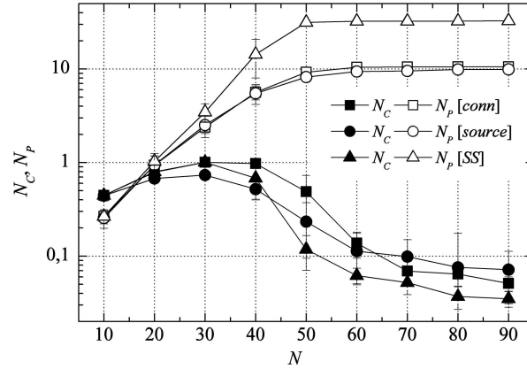
Fig. 7. Number of bandwidth requests (contention-based and piggybacked) per uplink subframe versus offered load.
