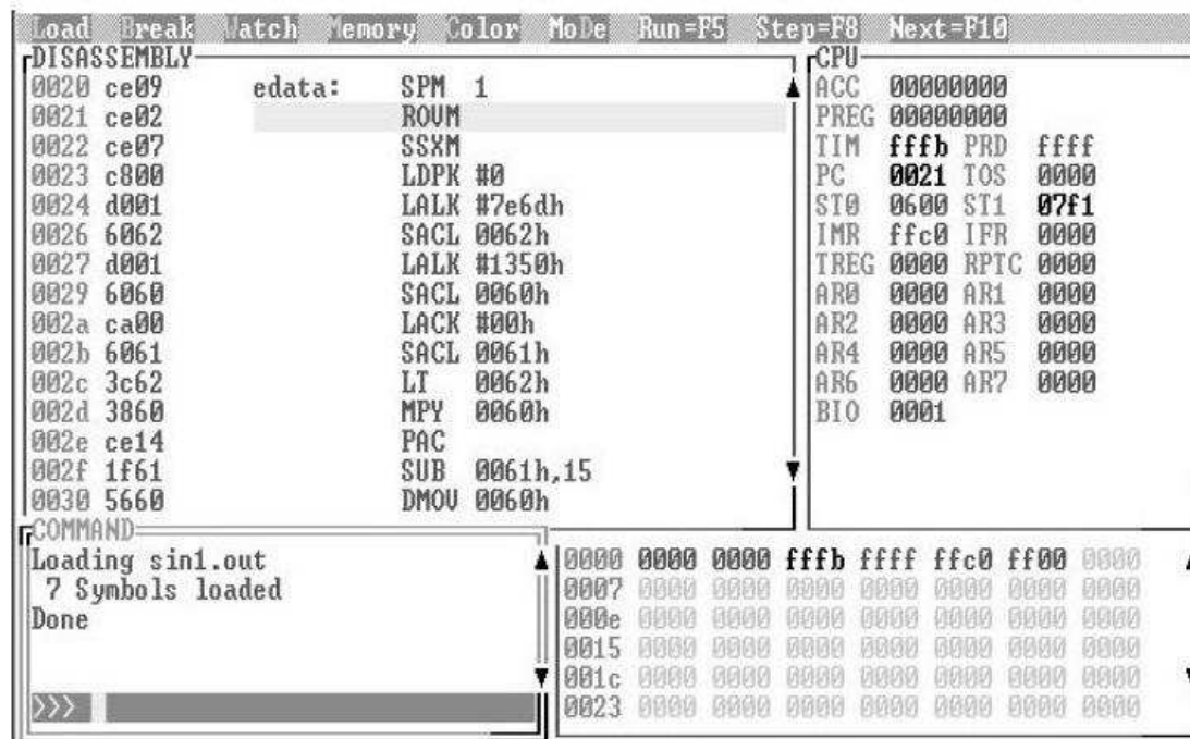
Fig. 2 sim2x Simulator's window
