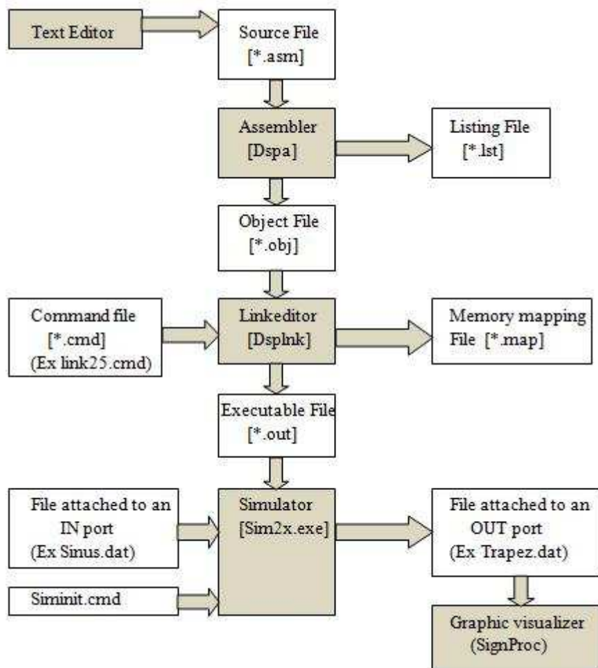
Fig. 1 Developing steps of an application for simulation
